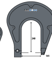
Riveting Arms HR210 & HR310 Ref: 064089
